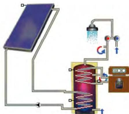
Figure 46: Hydraulic scheme of the DHW system for multi-family houses
