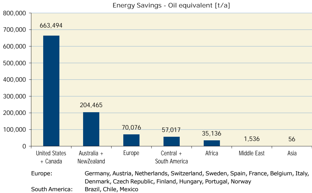
Figure 29: Annual energy savings in oil equivalents by unglazed water collectors in operation by economic region in 2009
